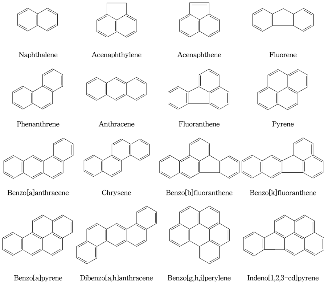
Fig. 1. Structure of EPA 16 PAHs.
